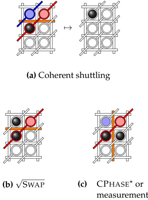
Figure 4.2. Schematic representation of the use of control lines for the native operations in the QDP. Qubits are represented by black balls on the grid. Red or blue colored dots are empty, but their dot potentials change due to an operation of the diagonal line they are coupled to. Empty dots, unaffected by grid operations, are white. (a) Vertical shuttling of a qubit (to the top left dot) requires to lower the orange barrier. One can then either raise the dot potentials on the red diagonal line, or lower the potential on the blue dot by pulsing the blue diagonal. (b) Schematic representation of the control lines used for performing two-qubit \sqrt{\text{SWAP}} gate between the two qubits on that grid. The orange barrier is lowered and the red diagonal line is utilized to detune dot potentials. (c) Grid operations necessary to perform a measurement or a two-qubit effective \text{CPHASE}^* gate between the two qubits. The orange barrier between the two qubits is lowered, and the dot potentials along the red diagonal line is raised by pulsing the latter. Note that the empty, red colored dot is also effected by that action, and its barrier to the adjacent dot is lowered. If the two dots in the upper row were not empty, side effects would occur. See Section 4.3.3.4 for more information on the nature of the two-qubit gates. Note also that the readout procedure of the measurement requires us to have the upper dot (light blue) empty, if the barrier gate between them is used for readout.
